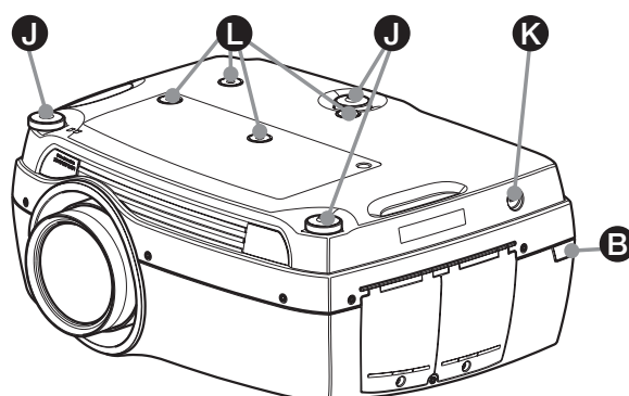
Figure 4-3. - Projector bottom view
