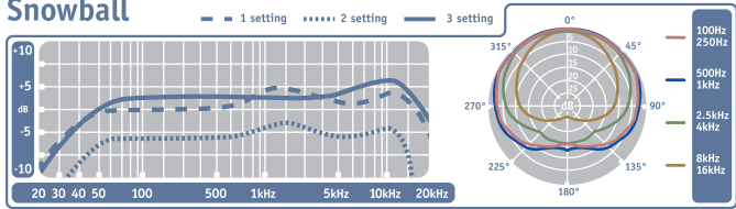
Frequency Response
