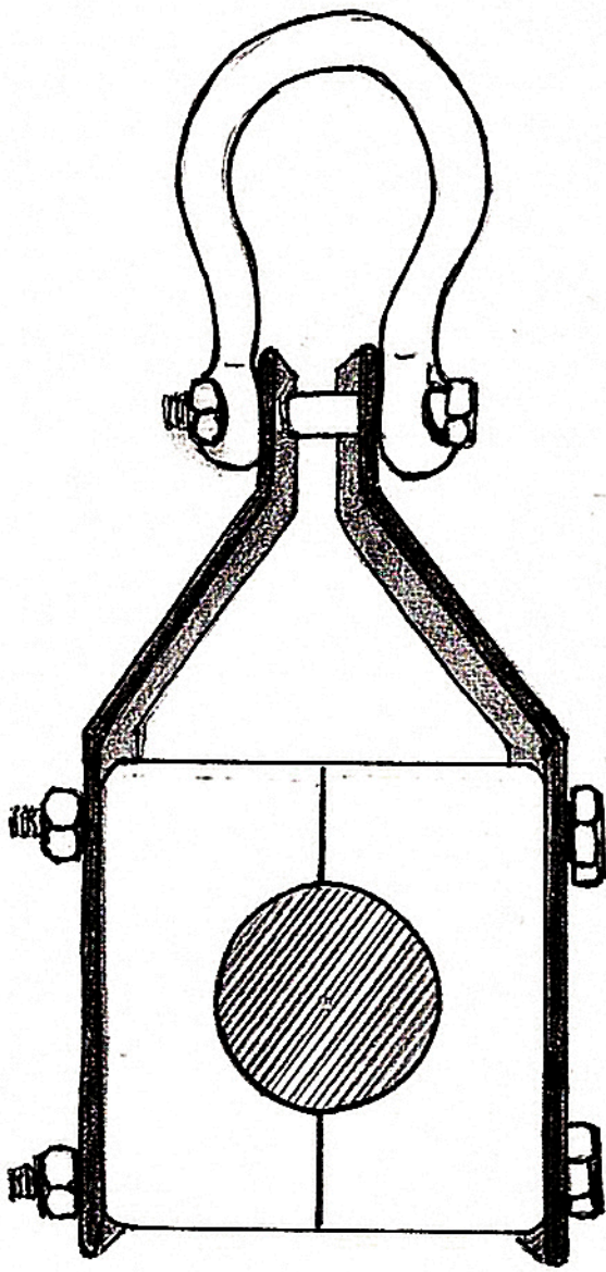
HANGING BRACKET FOR A MODULAR F2 PART # 4960 (4 TO A SET)
