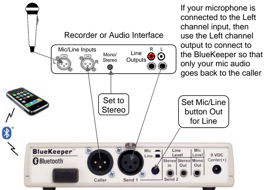
Figure 7: Stereo Output Interface
