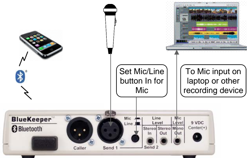
Figure 6: Mono Output to Recorder
