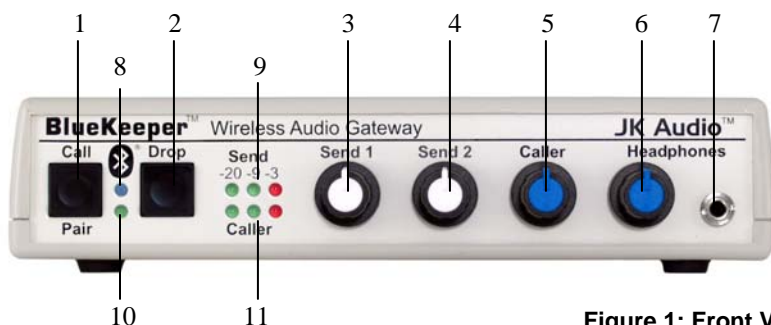
Figure 1: Front View
