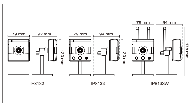
Dimension
