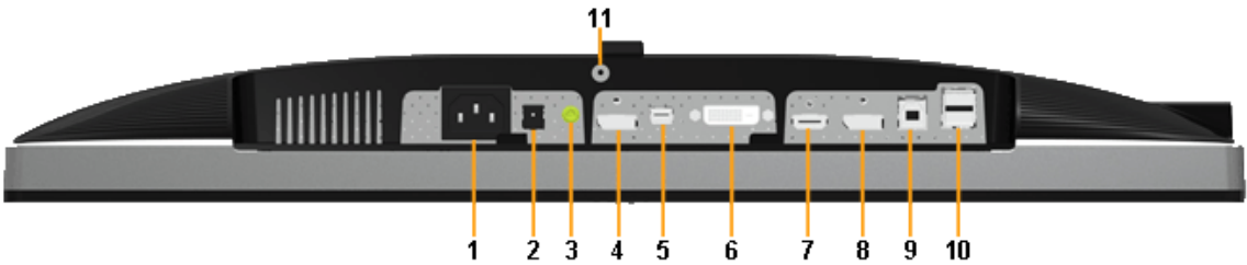
Bottom view without monitor stand
