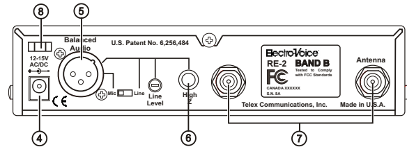
Figure 2 - RE-2 Back Panel
