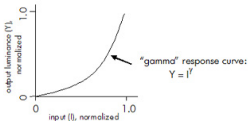
Figure A-6 Gamma Curve Response Characteristic
