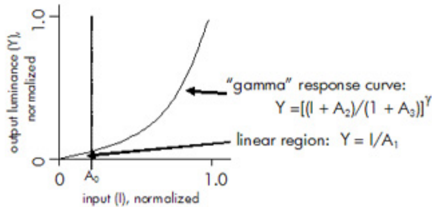
Figure A-7 Low Linear Region Response Curve
