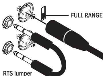
TRS jumper between CH 1 and CH 2.
